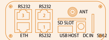
DIAGRAM: PORTS CONNECTION
